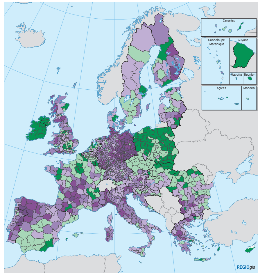
Map 2.4 Median age in NUTS 3 regions, 2016 Median age, in years 0 – 40 40 – 42.5 42.5 – 45 45 – 47.5 47.5 – 50 50+ EU-28 = 42.6 years Source: Eurostat 0 500 km © EuroGeographics Association for the administrative boundaries
