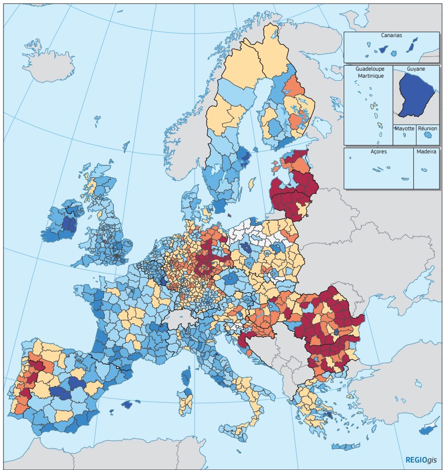
Map 2.3 Total population change in NUTS 3 regions, 2005–2015 Total change (%) < -10 5 – 10 -10 – -5 10 – 15 -5 – 0 > 15 0 – 5 no data EU-28 = 2.84 DK, DE, DED, DEE: data before 2007 was extrapolated. PLS2: NUTS 2 Source: Eurostat, DG REGIO 0 500 km © EuroGeographics Association for the administrative boundaries
